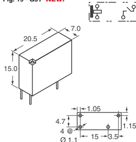
Fig. 19 - G5T NEW!
